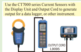
DISPLAY UNIT CM7290, CM7291 For CT7000 series, CM7291 with built-in Bluetooth® wireless technology
